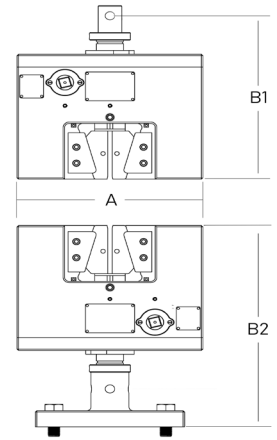
2716-028 Grip Dimensions
